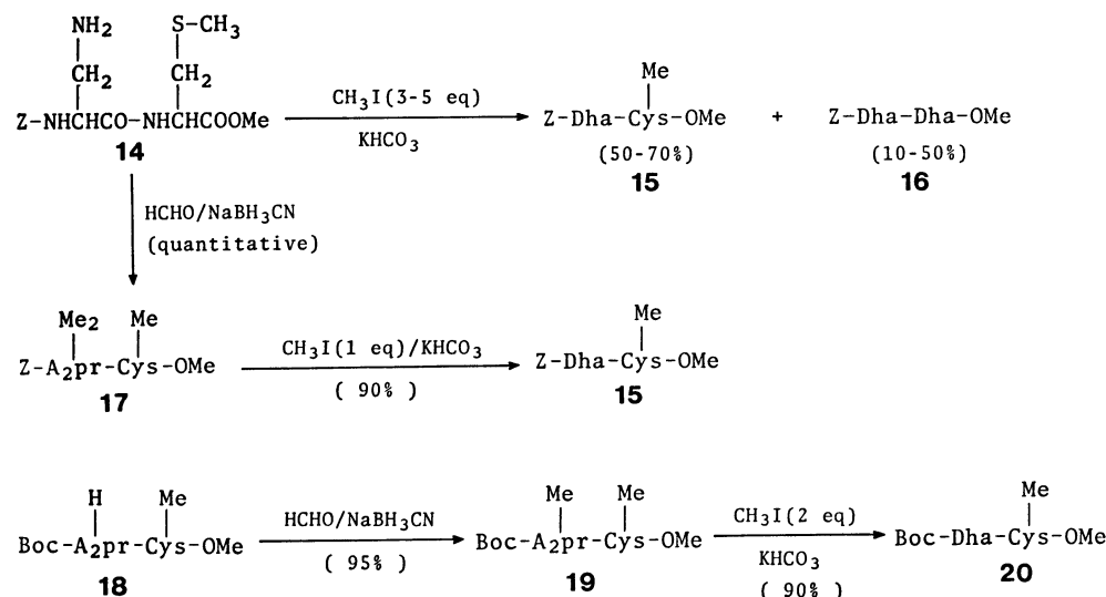
Fig. 7. An improved method of the dehydroalanine synthesis through Hofmann degradation via the N^{\beta} -methyl derivative of A_2\text{pr} residue.
